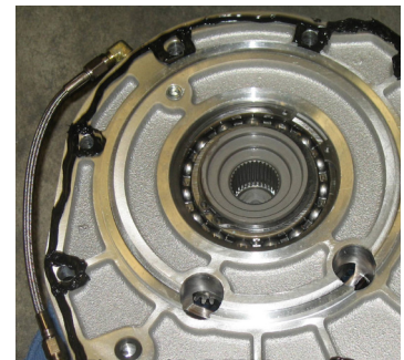
Figure 15: RTV Pattern
