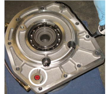
Figure 14: Plug/O-ring location
