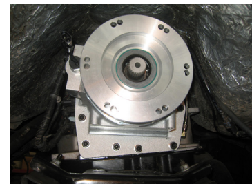
Figure 16: RubiCrawler Installed
