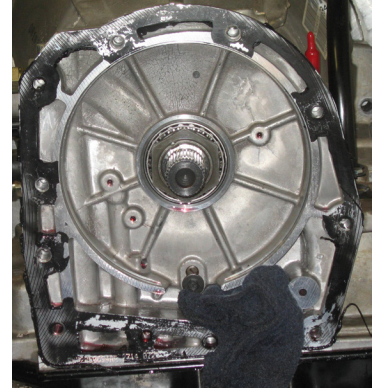
Figure 5: Rag Placement
